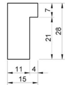
profile dimensions
